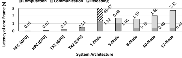
Fig. 13: Measured end-to-end latency of one frame.
